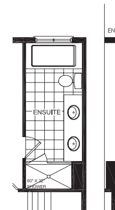
EXECUTIVE ENSUITE (3 BEDROOM PLAN ONLY)
