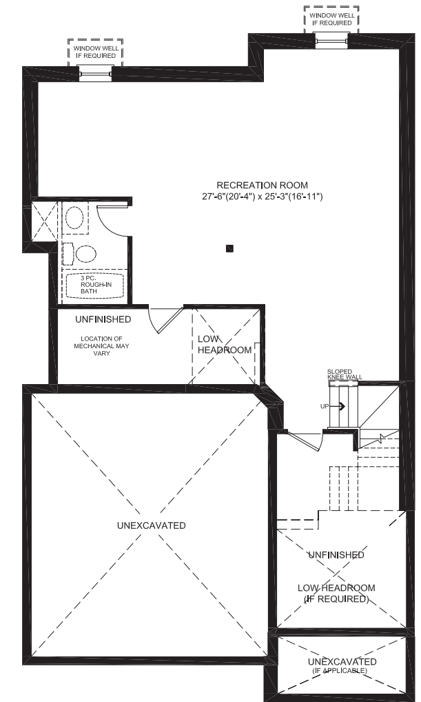
FINISHED BASEMENT
