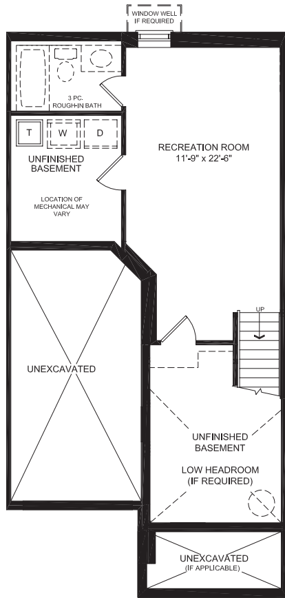
FINISHED BASEMENT
