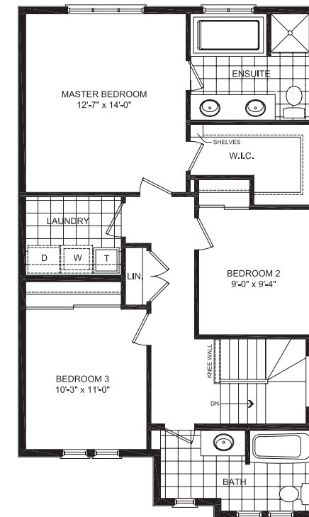
SECOND FLOOR W/ EXECUTIVE ENSUITE
