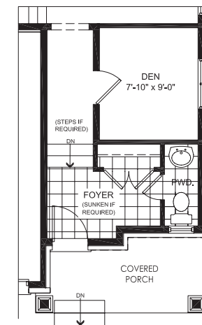
GROUND FLOOR DEN & FOYER
