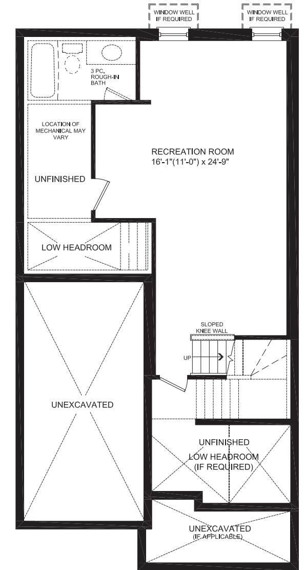
FINISHED BASEMENT
