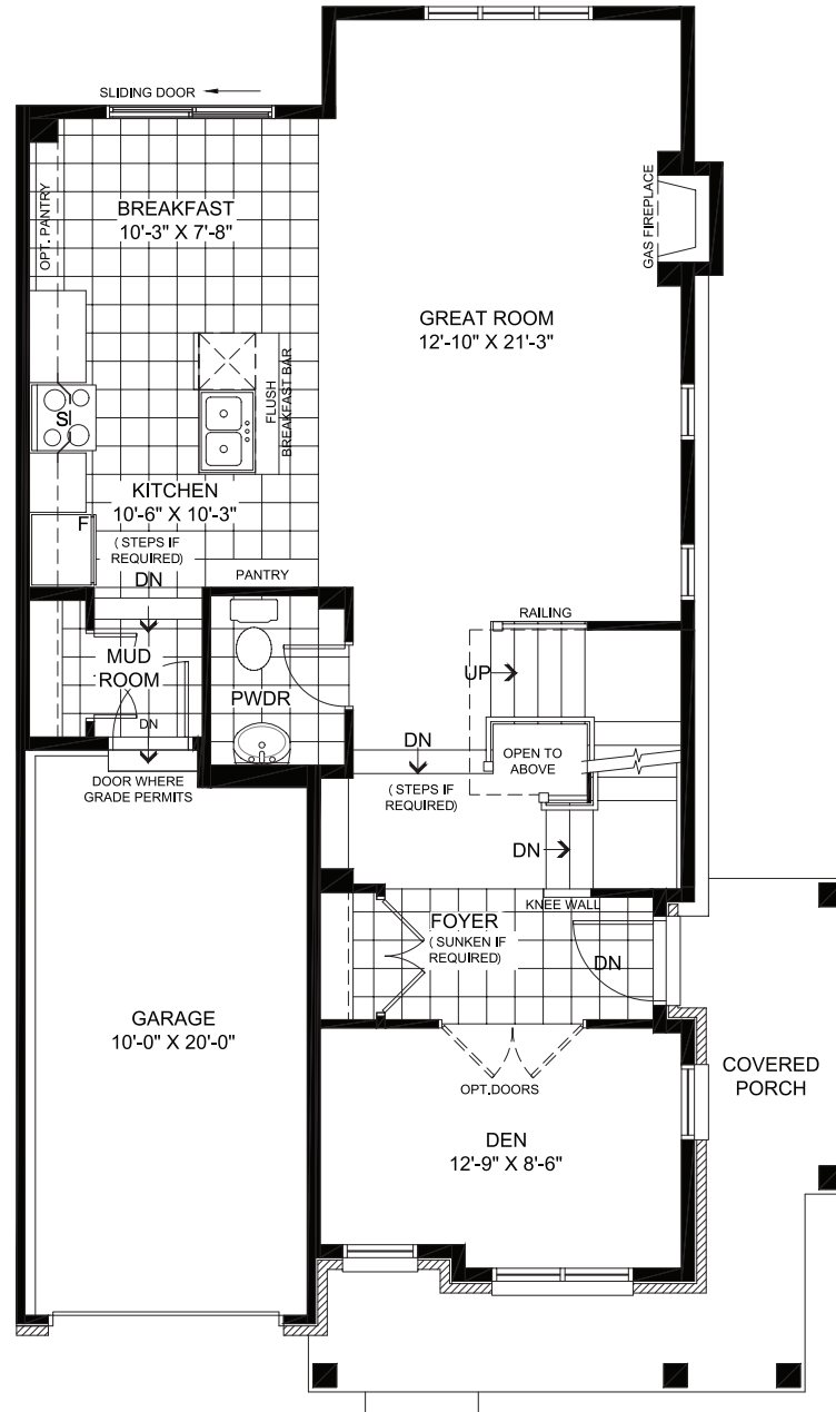
ALTERNATE GROUND FLOOR
