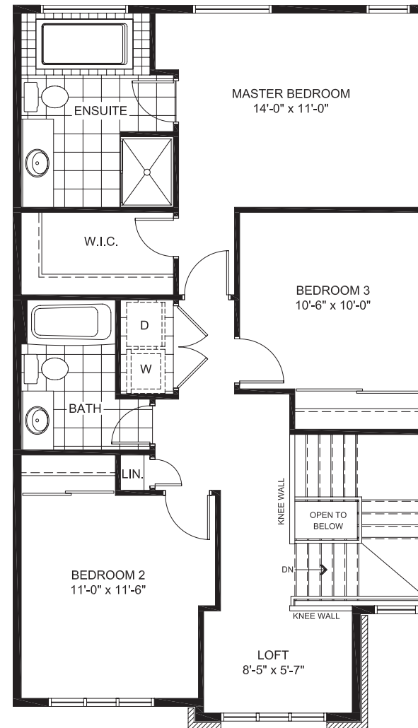
SECOND FLOOR
