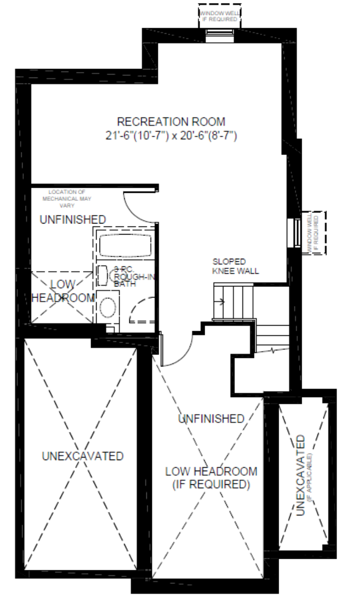
FINISHED BASEMENT
