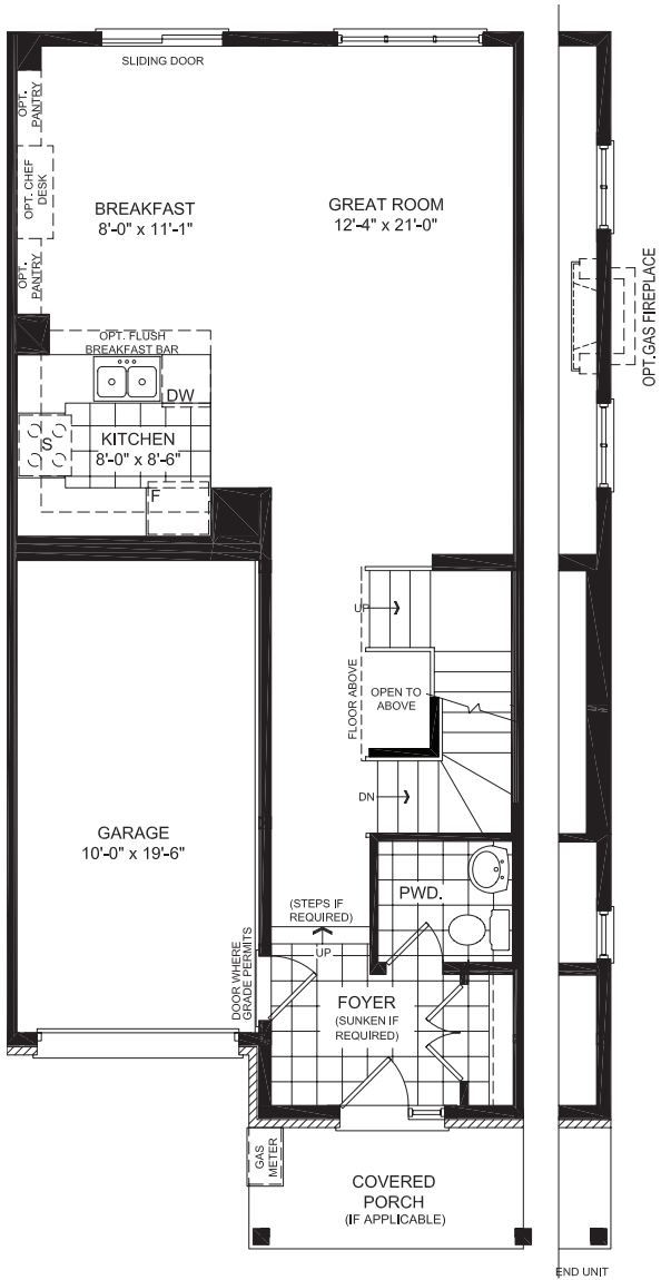
GROUND FLOOR
