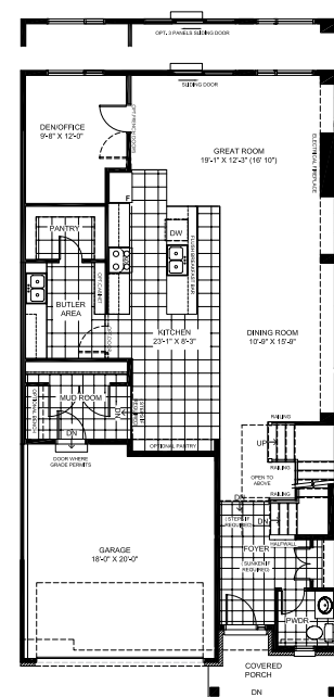
OPTIONAL GROUND FLOOR
