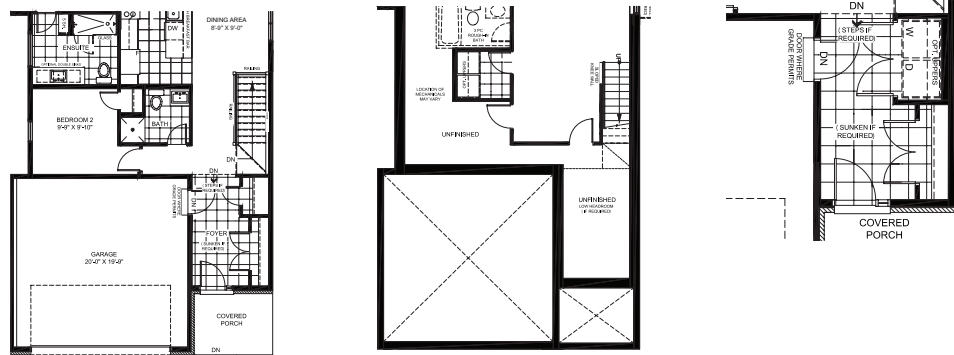
ALTERNATE GROUND FLOOR W/ LAUNDRY IN THE BASEMENT OR FOYER
