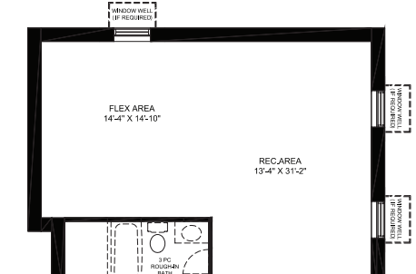
FINISHED REC AREA W/ FLEX SPACE
