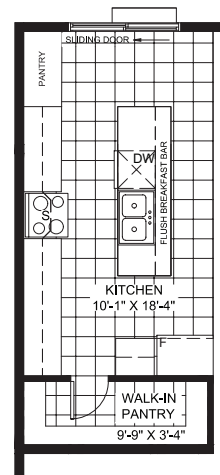
CHEF'S KITCHEN
