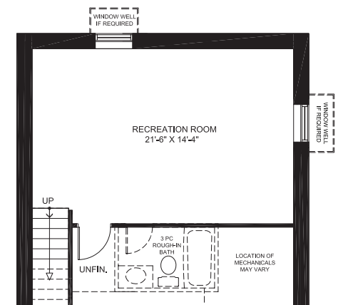
OPTIONAL FINISHED FLEX AREA
