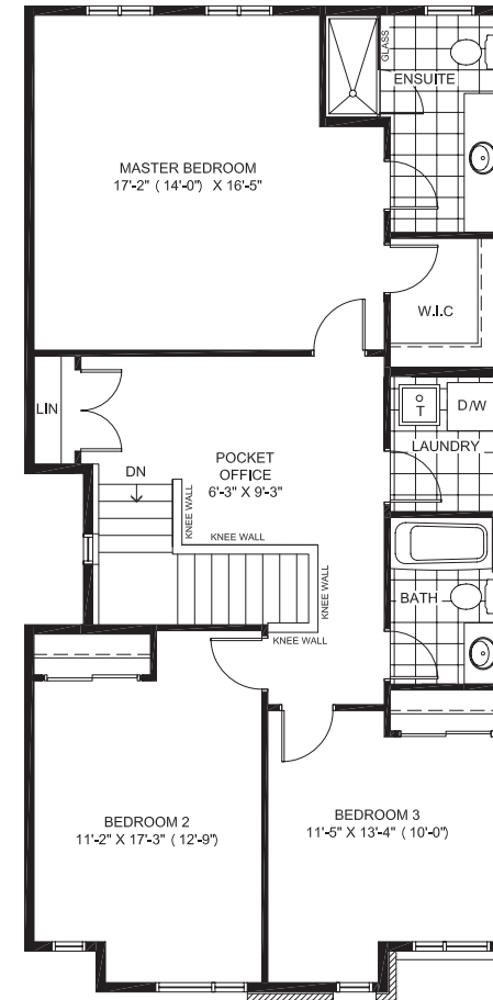
SECOND FLOOR
