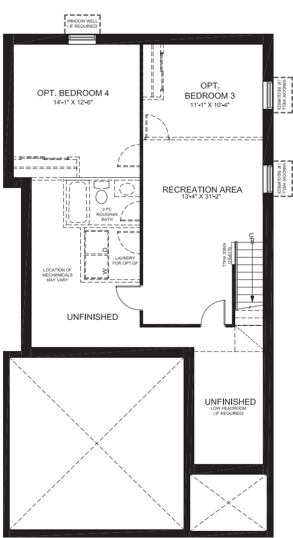
FINISHED BASEMENT
