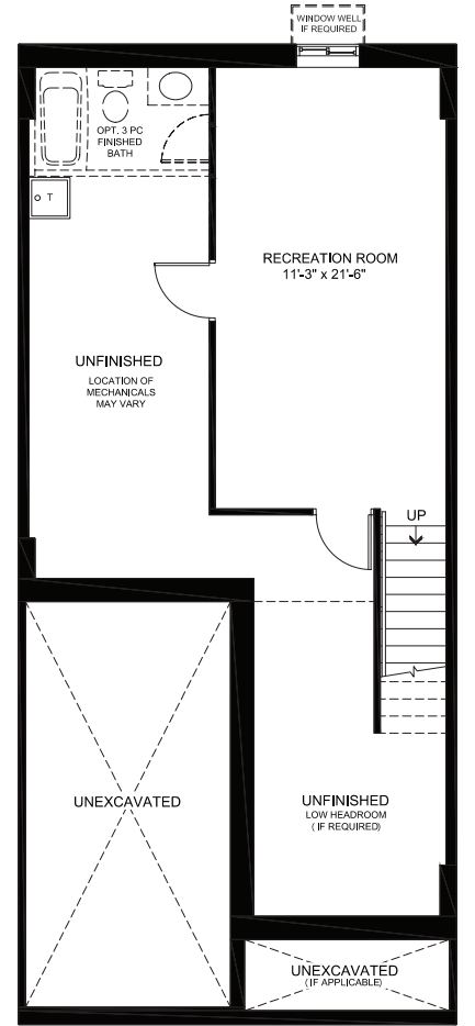
FINISHED BASEMENT
