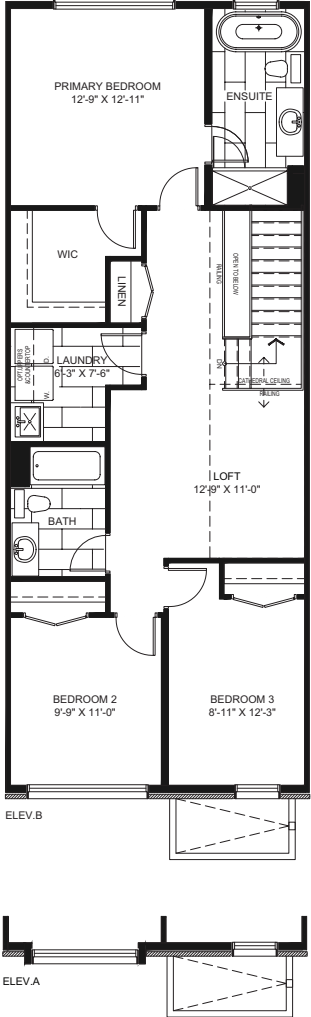
SECOND FLOOR
