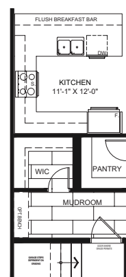
OPTIONAL GROUND FLOOR
