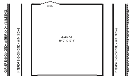
DETACHED DOUBLE-CAR GARAGE
