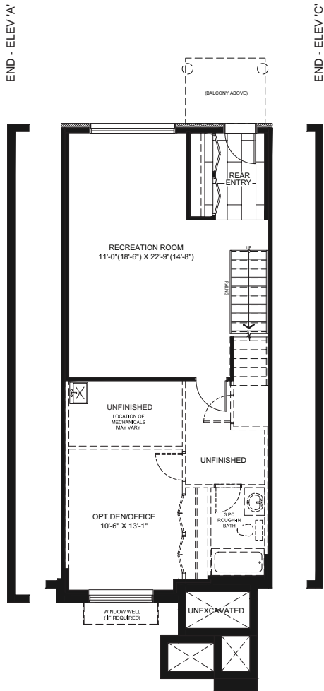
BASEMENT
